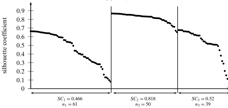
(b) k = 3, SC = 0.598
