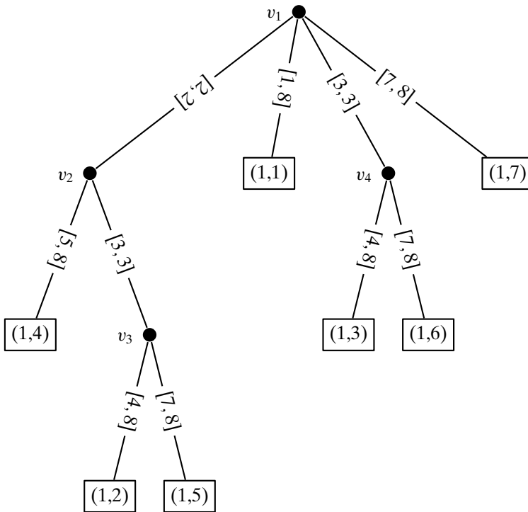
Figure 10.6. Suffix tree for s_1 = CAGAAGT\$ using edge-compression.
