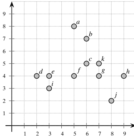
Figure 14.5. Dataset for Q2.
