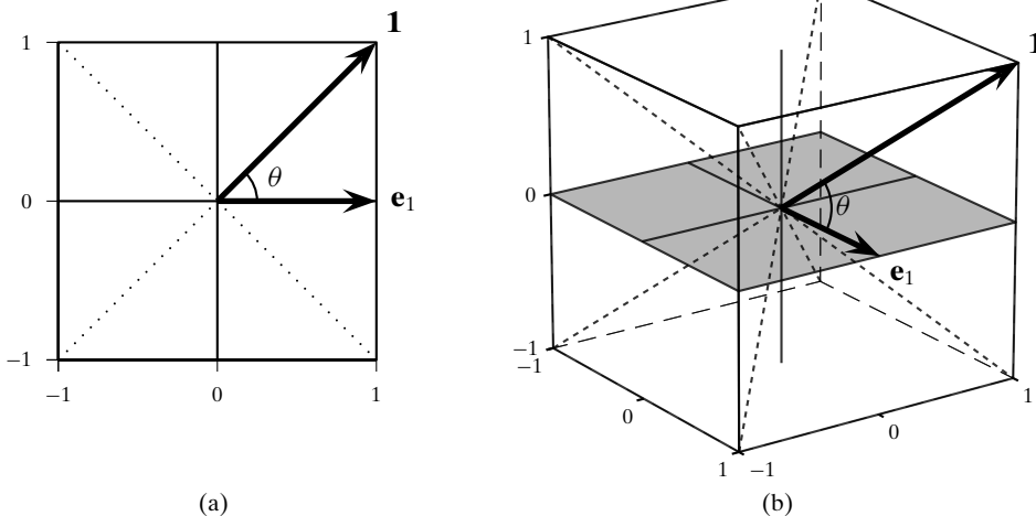
Figure 6.6. Angle between diagonal vector \mathbf{1} and \mathbf{e}_1 : in (a) two and (b) three dimensions.
