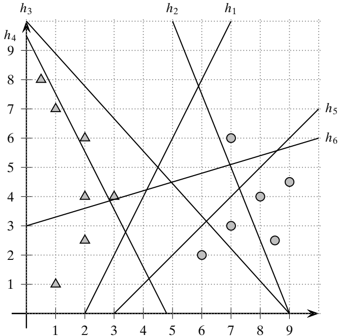
Figure 22.10. For Q4.
