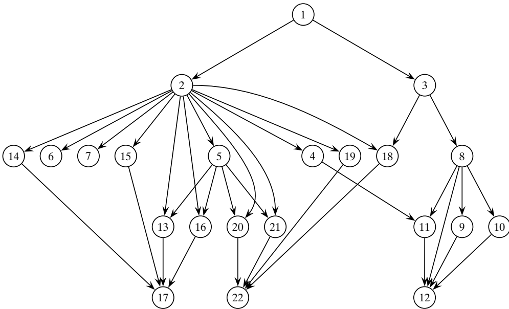
Figure 0.1. Chapter dependencies
