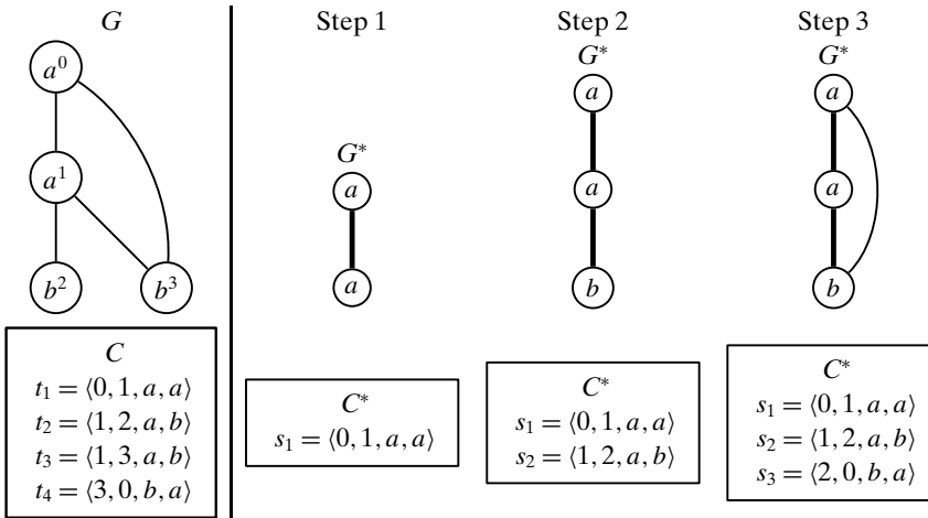
Figure 11.11. Canonicality checking.
