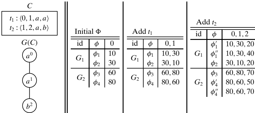
Figure 11.10. Subgraph isomorphisms.
