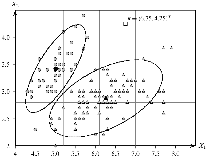
Figure 18.1. Iris data: X_1 :sepal length versus X_2 :sepal width. The class means are show in black; the density contours are also shown. The square represents a test point labeled \mathbf{x} .
