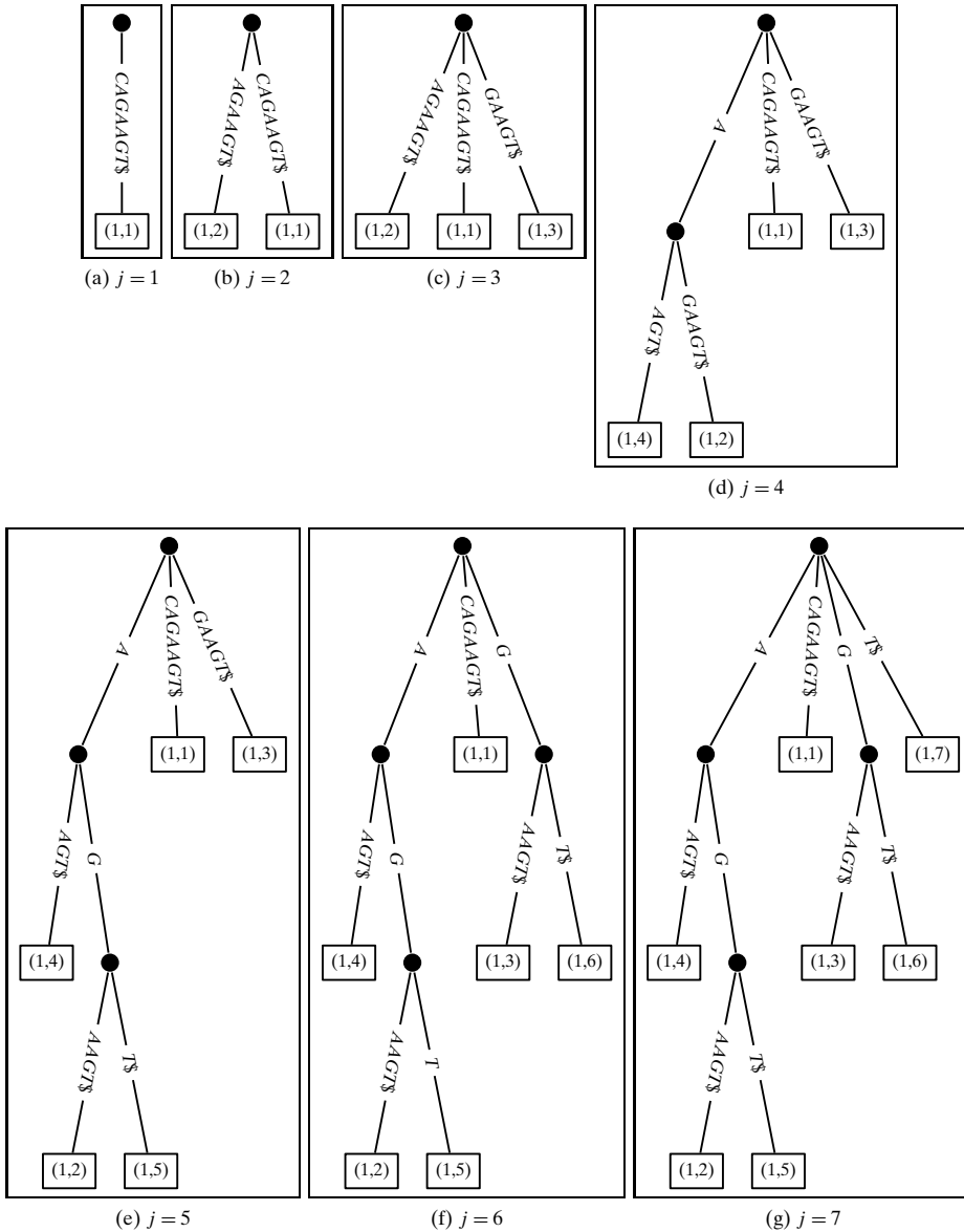
Figure 10.4. Suffix tree construction: (a)–(g) show the successive changes to the tree, after we add the j th suffix of s_1 = CAGAAGT\$ for j = 1, \dots, 7 .
