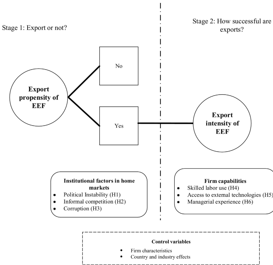
Fig. 1. Conceptual framework.
