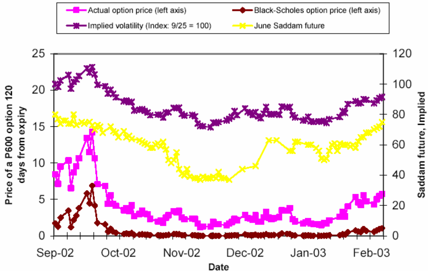
Figure 6. Probability of war and the prices of out-of-the-money puts on the S&P 500
