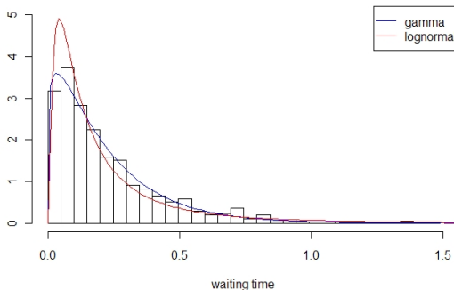
Parametric fits for waiting times
