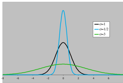
Same mean, different standard deviations
