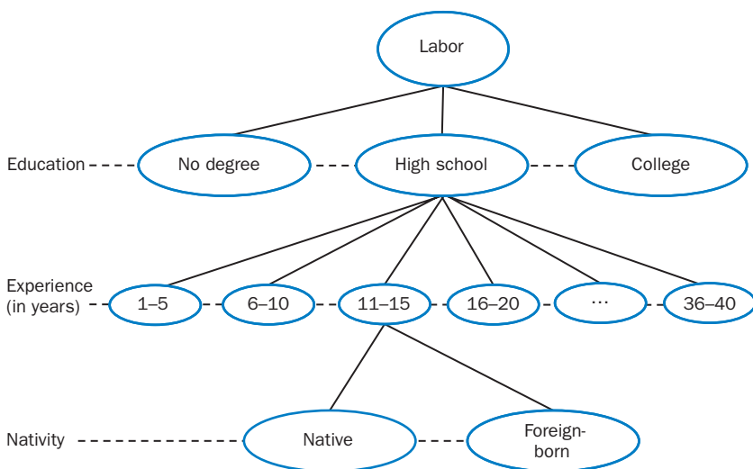
Figure 3A.1 The nested constant elasticity of substitution production function
